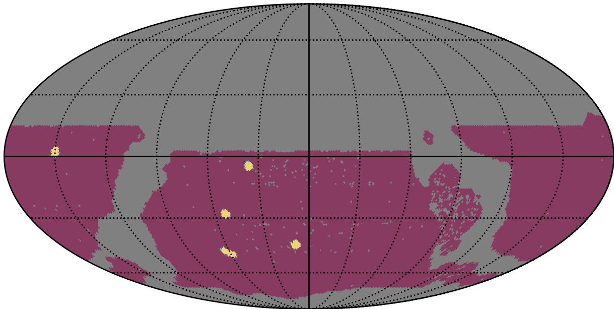
early_u_fpextra3.0_v3.4_10yrs WFD: NumberOfQuickRevisits
