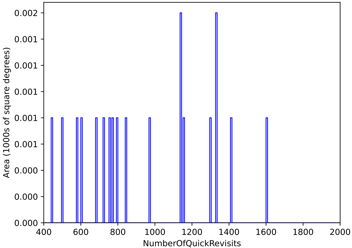
early_u_fpextra3.0_v3.4_10yrs WFD: NumberOfQuickRevisits
