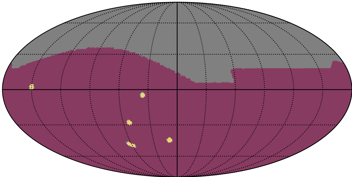
early_u_fpextra3.0_v3.4_10yrs All sky: NumberOfQuickRevisits
