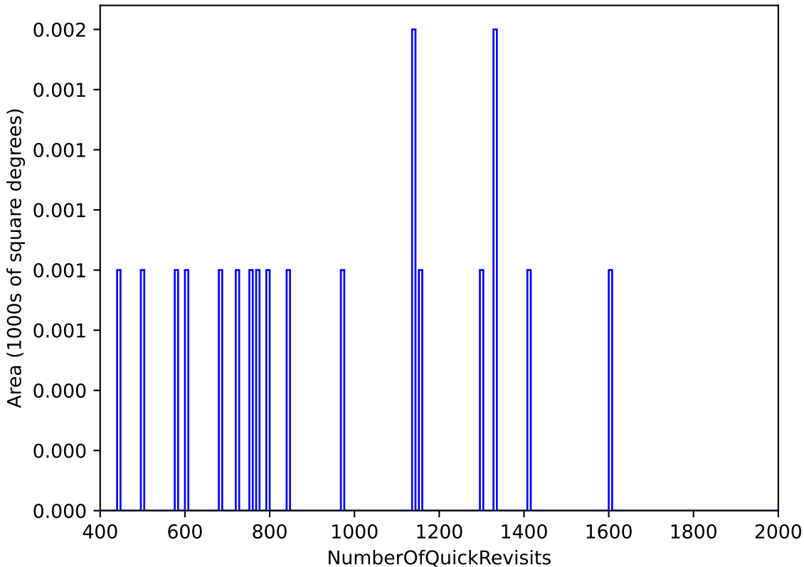
early_u_fpextra3.0_v3.4_10yrs All sky: NumberOfQuickRevisits
