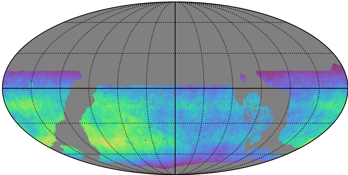
early_u_fpextra3.0_v3.4_10yrs WFD z band: Normalized Teff
