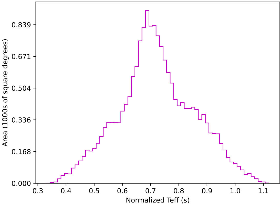
early_u_fpextra3.0_v3.4_10yrs WFD z band: Normalized Teff
