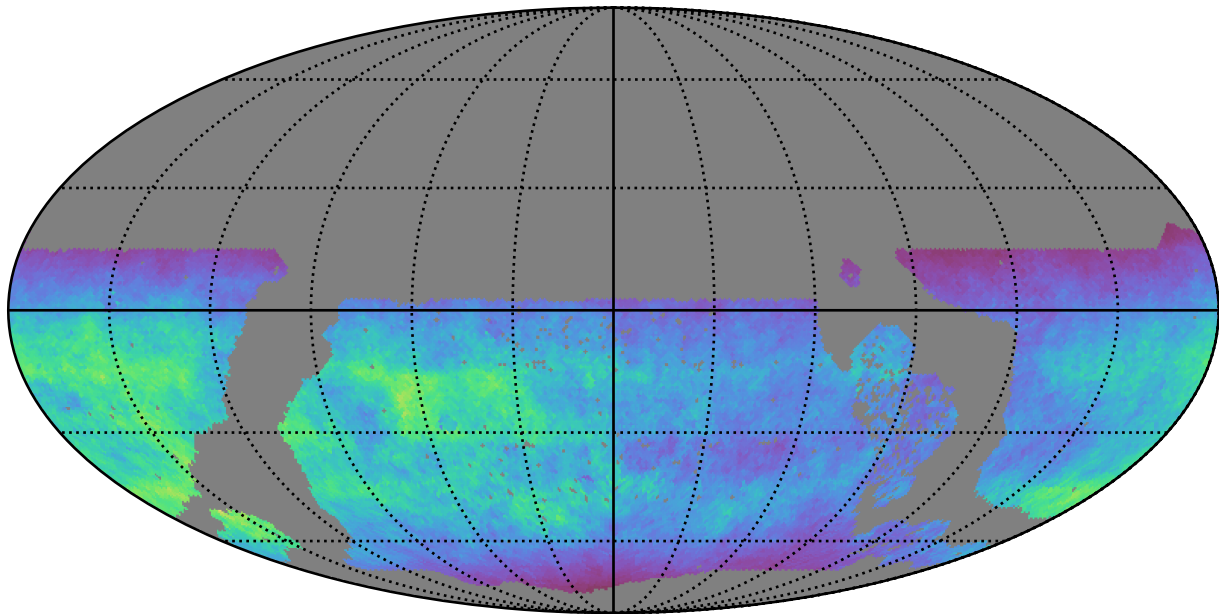
early_u_fpextra3.0_v3.4_10yrs WFD u band: Normalized Teff
