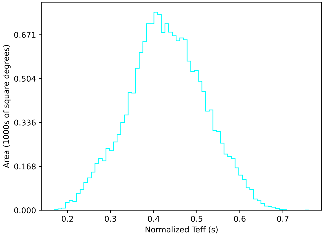
early_u_fpextra3.0_v3.4_10yrs WFD u band: Normalized Teff
