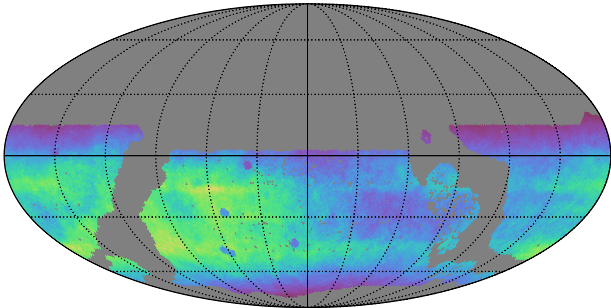
early_u_fpextra3.0_v3.4_10yrs WFD r band: Normalized Teff
