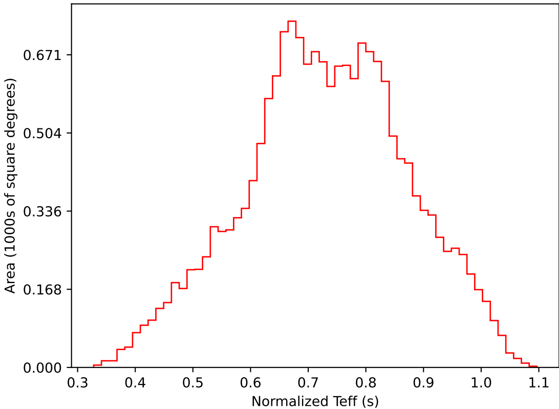
early_u_fpextra3.0_v3.4_10yrs WFD i band: Normalized Teff
