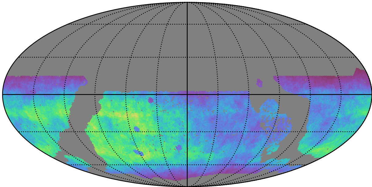
early_u_fpextra3.0_v3.4_10yrs WFD g band: Normalized Teff
