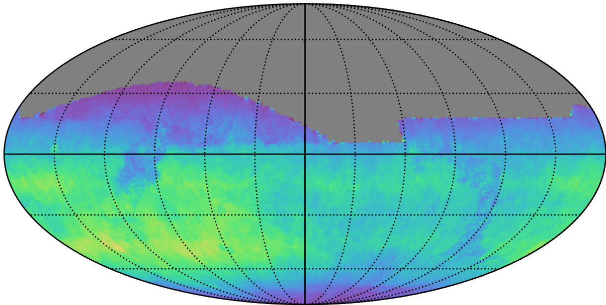
early_u_fpextra3.0_v3.4_10yrs All sky z band: Normalized Teff
