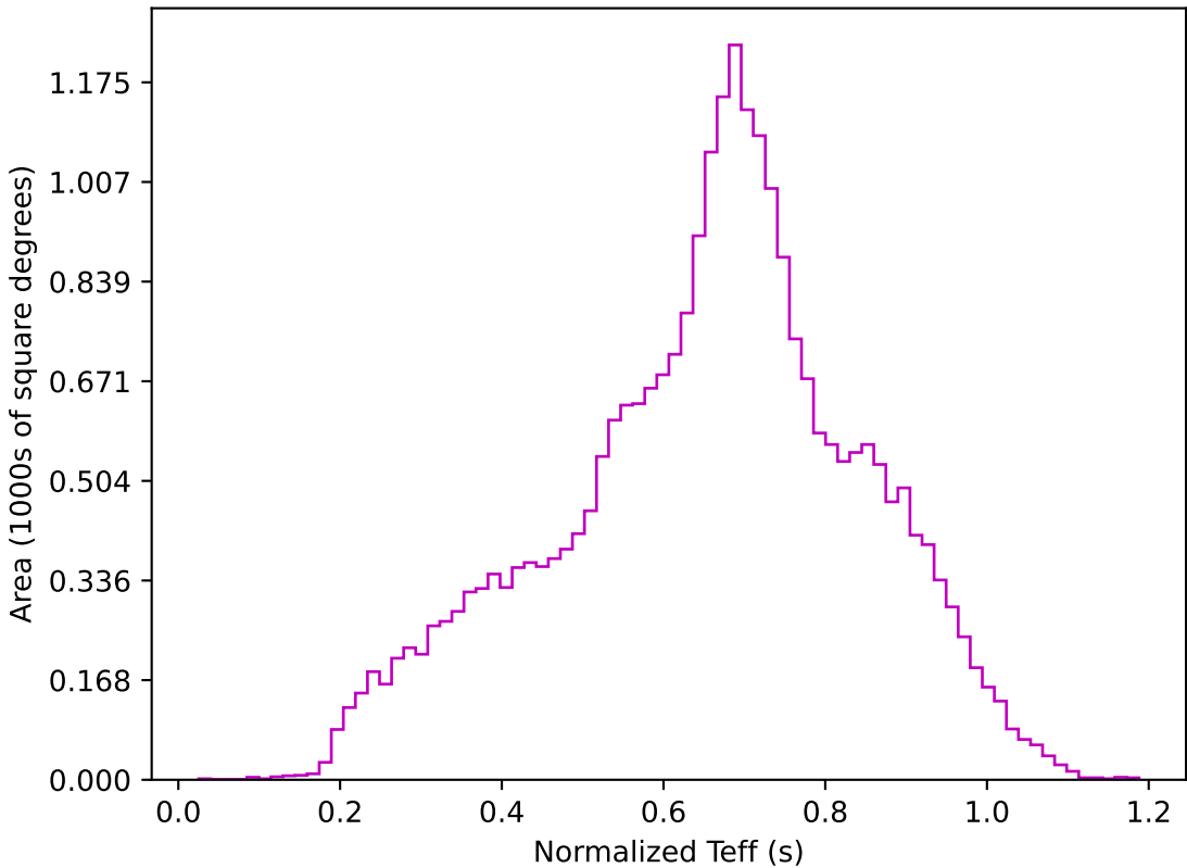
early_u_fpextra3.0_v3.4_10yrs All sky z band: Normalized Teff
