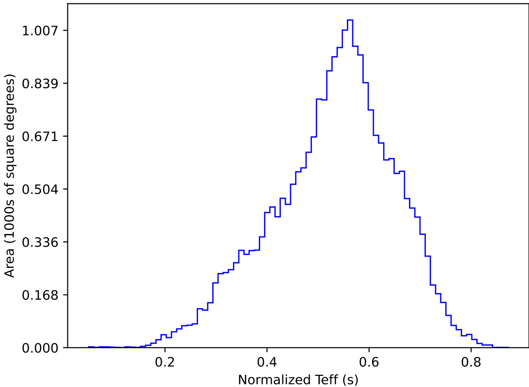
early_u_fpextra3.0_v3.4_10yrs All sky y band: Normalized Teff
