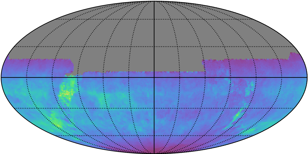
early_u_fpextra3.0_v3.4_10yrs All sky u band: Normalized Teff
