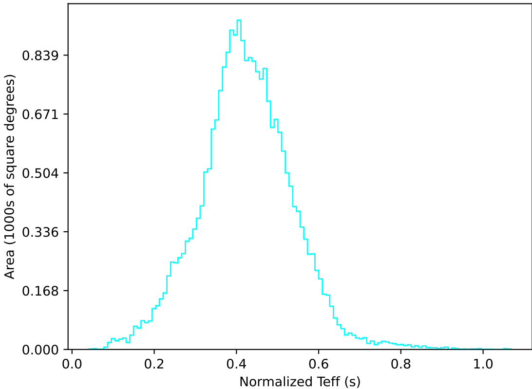
early_u_fpextra3.0_v3.4_10yrs All sky u band: Normalized Teff
