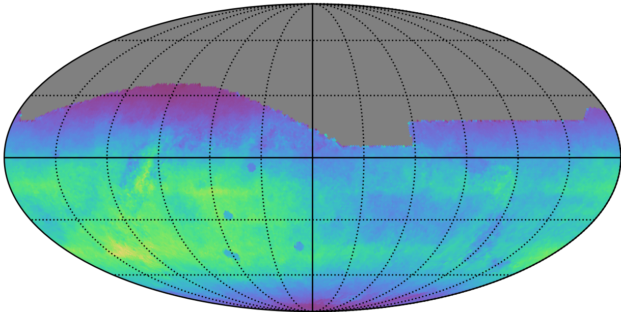
early_u_fpextra3.0_v3.4_10yrs All sky r band: Normalized Teff
