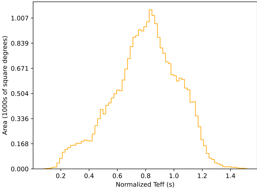
early_u_fpextra3.0_v3.4_10yrs All sky r band: Normalized Teff
