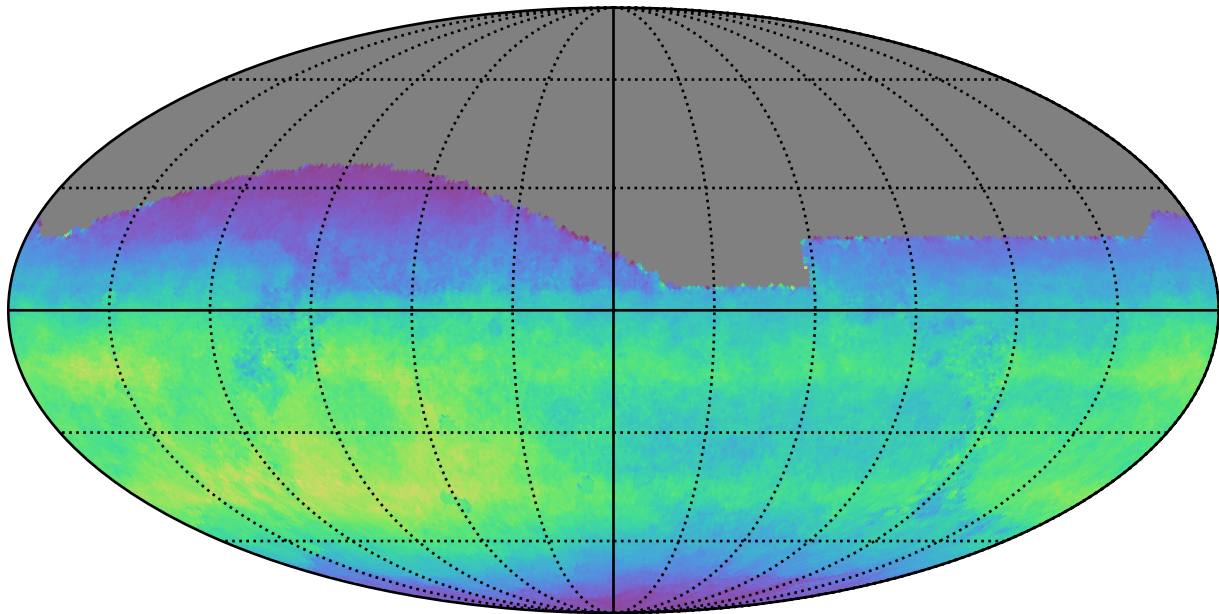
early_u_fpextra3.0_v3.4_10yrs All sky i band: Normalized Teff
