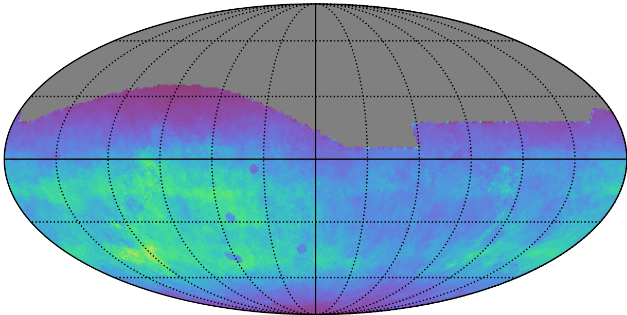
early_u_fpextra3.0_v3.4_10yrs All sky g band: Normalized Teff
