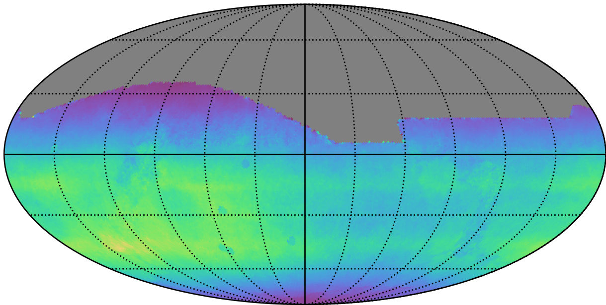
early_u_fpextra3.0_v3.4_10yrs All sky all bands: Normalized Teff
