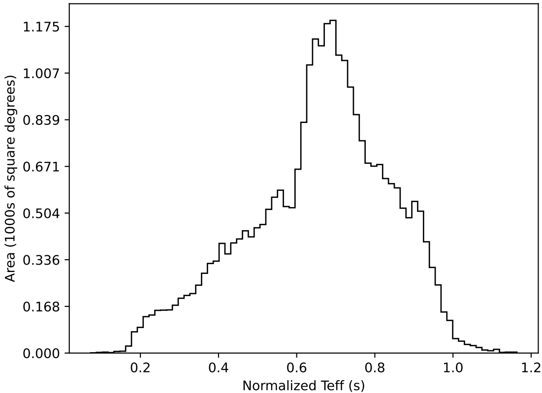
early_u_fpextra3.0_v3.4_10yrs All sky all bands: Normalized Teff
