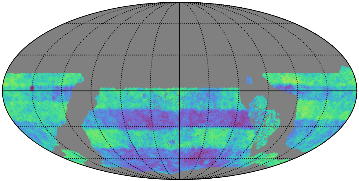
early_u_fpextra3.0_v3.4_10yrs WFD: Normalized Proper Motion Uncert @ 24.0
