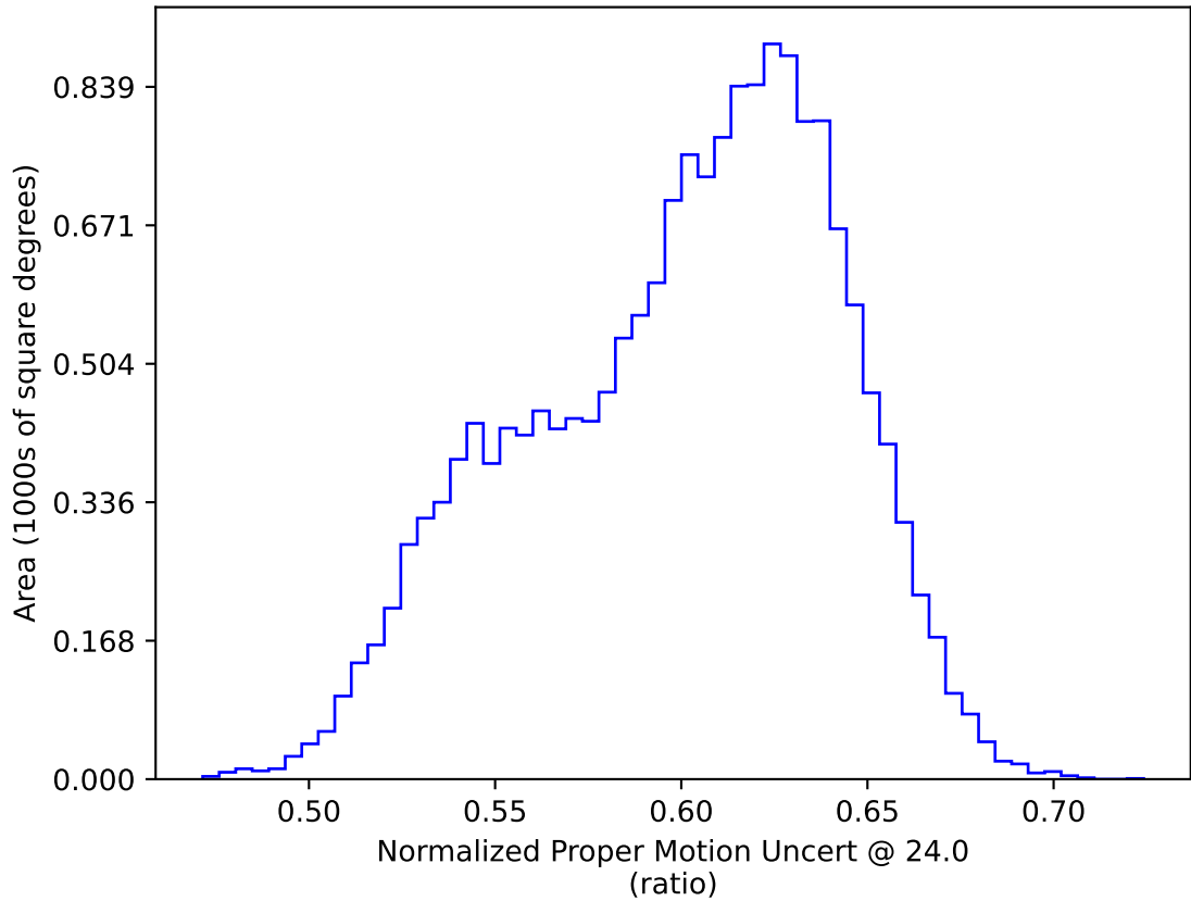
early_u_fpextra3.0_v3.4_10yrs WFD: Normalized Proper Motion Uncert @ 24.0
