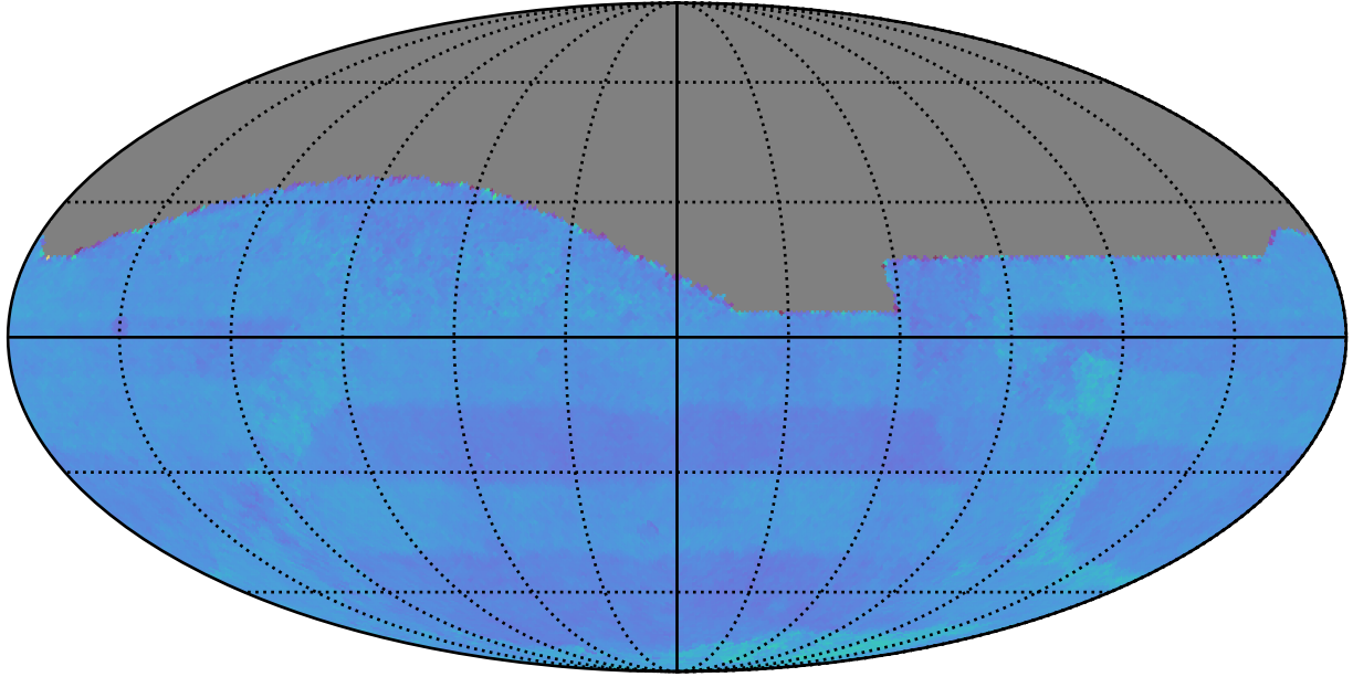
early_u_fpextra3.0_v3.4_10yrs All sky: Normalized Proper Motion Uncert @ 24.0
