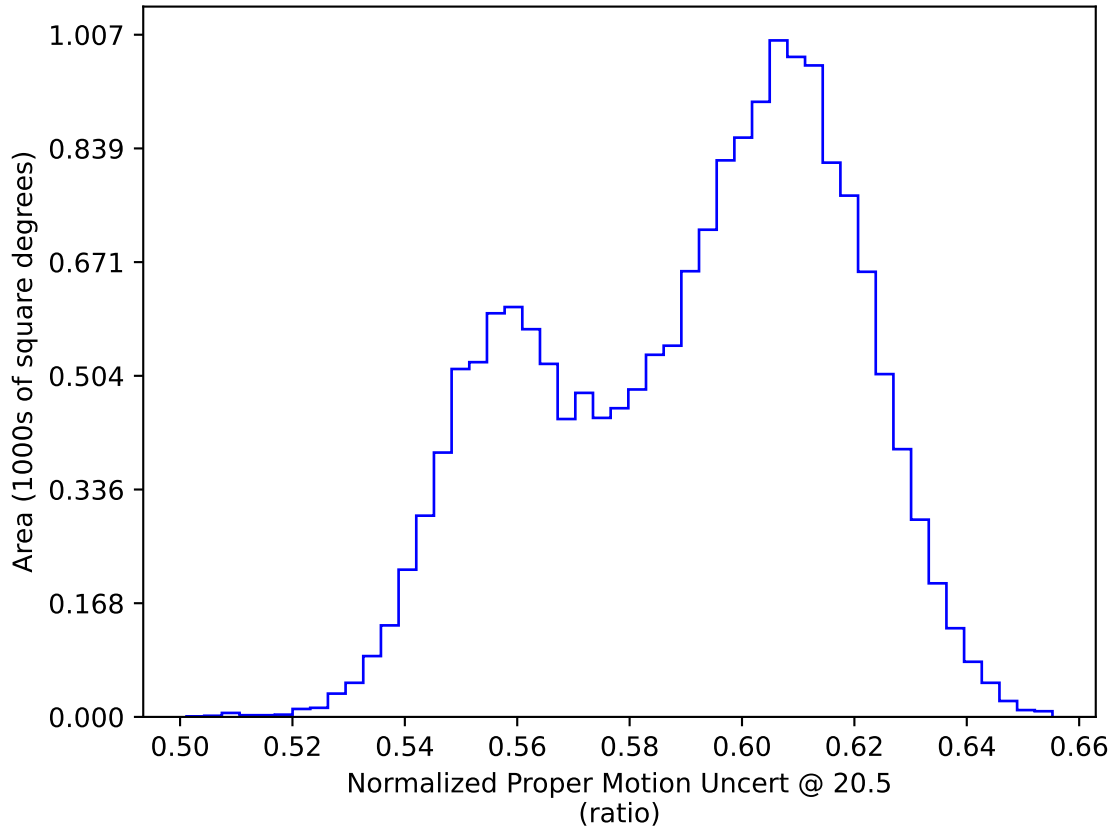
early_u_fpextra3.0_v3.4_10yrs WFD: Normalized Proper Motion Uncert @ 20.5
