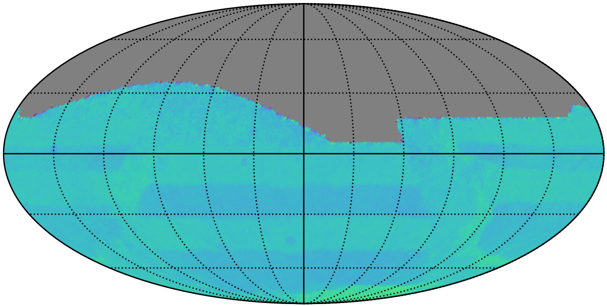
early_u_fpextra3.0_v3.4_10yrs All sky: Normalized Proper Motion Uncert @ 20.5
