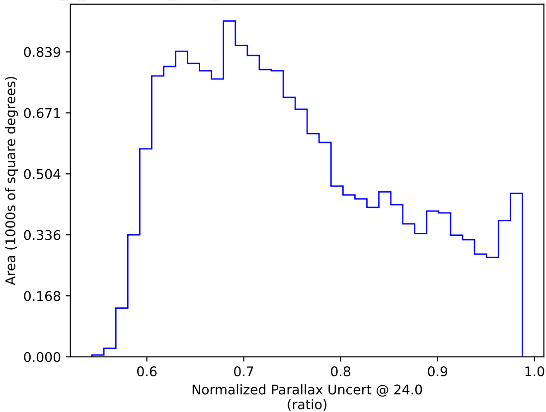
early_u_fpextra3.0_v3.4_10yrs WFD: Normalized Parallax Uncert @ 24.0
