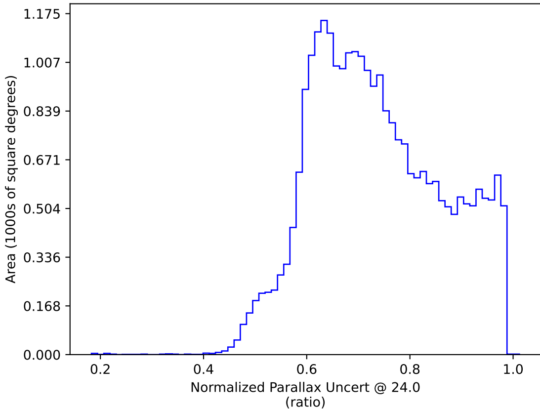
early_u_fpextra3.0_v3.4_10yrs All sky: Normalized Parallax Uncert @ 24.0
