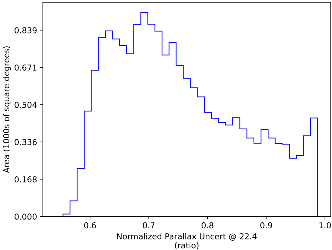
early_u_fpextra3.0_v3.4_10yrs WFD: Normalized Parallax Uncert @ 22.4
