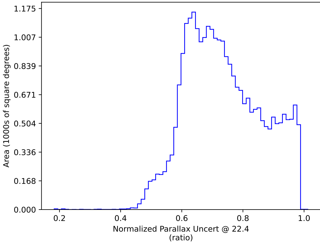
early_u_fpextra3.0_v3.4_10yrs All sky: Normalized Parallax Uncert @ 22.4
