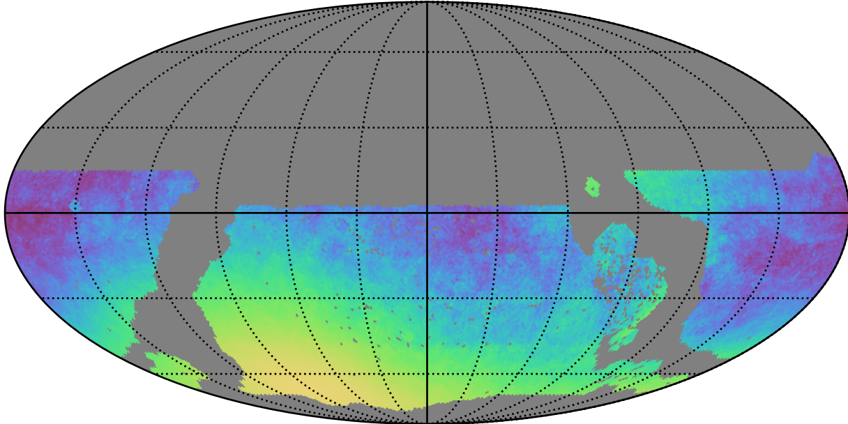
early_u_fpextra3.0_v3.4_10yrs WFD y band only: Normalized Parallax Uncert @ 21.3
