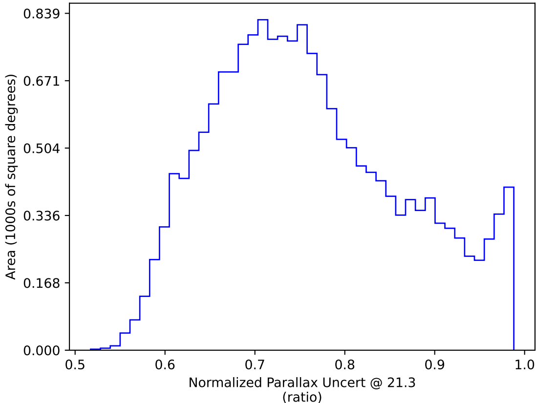
early_u_fpextra3.0_v3.4_10yrs WFD y band only: Normalized Parallax Uncert @ 21.3
