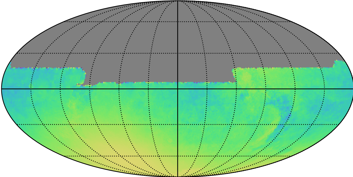
early_u_fpextra3.0_v3.4_10yrs All sky y band only: Normalized Parallax Uncert @ 21.3
