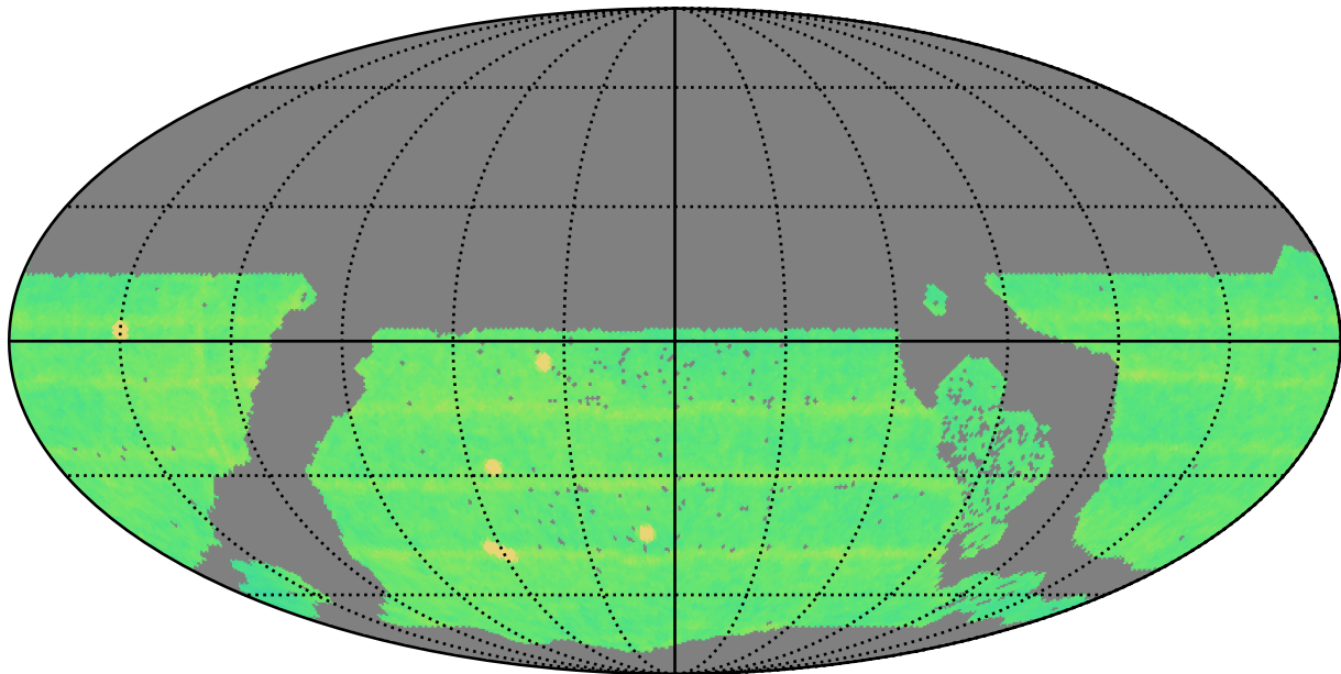
early_u_fpextra3.0_v3.4_10yrs WFD all bands: N Unique Nights
