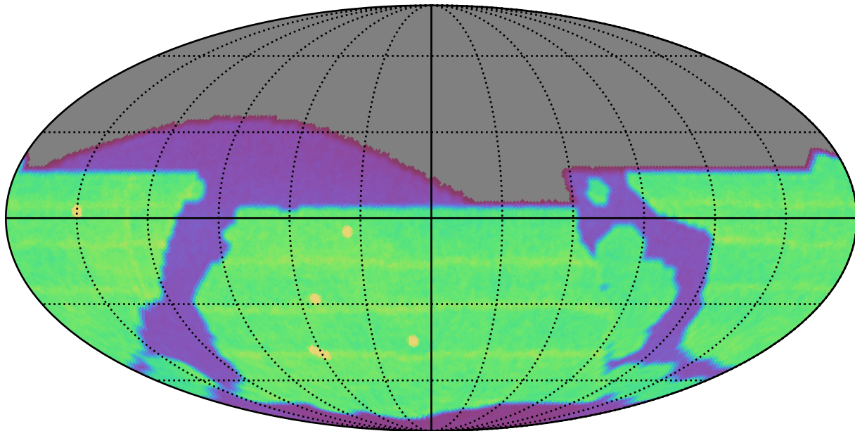
early_u_fpextra3.0_v3.4_10yrs All sky all bands: N Unique Nights
