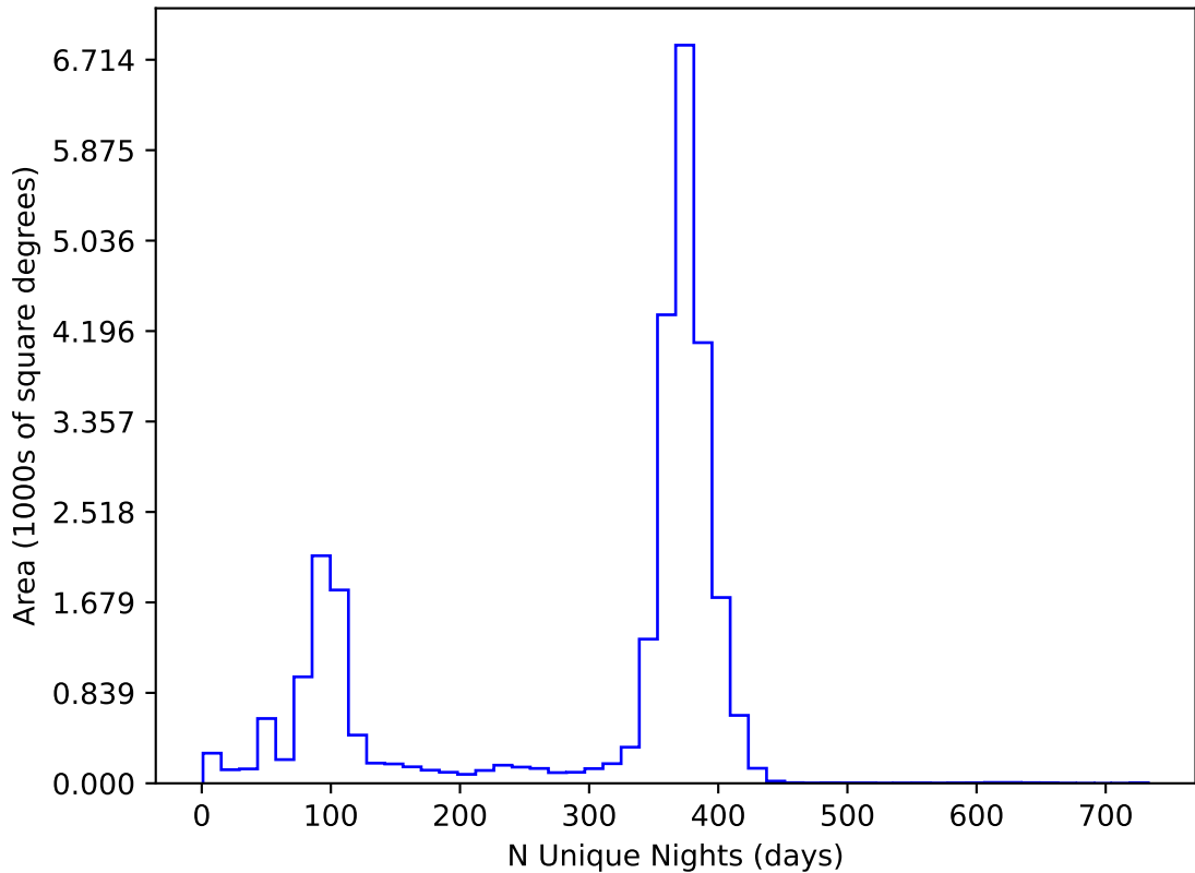
early_u_fpextra3.0_v3.4_10yrs All sky all bands: N Unique Nights
