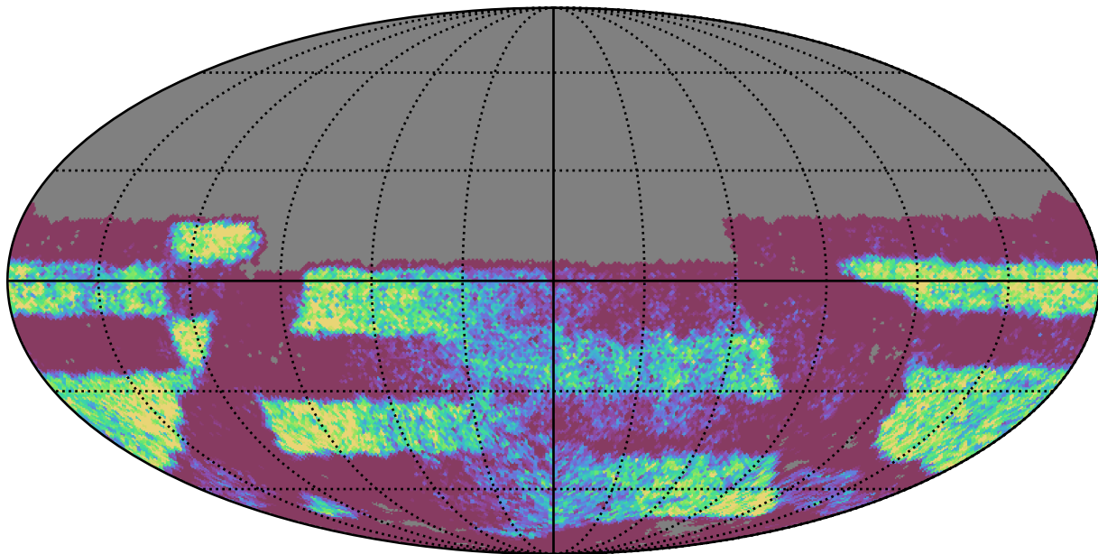
early_u_fpextra3.0_v3.4_10yrs Yr 3-4 y band: NVisits
