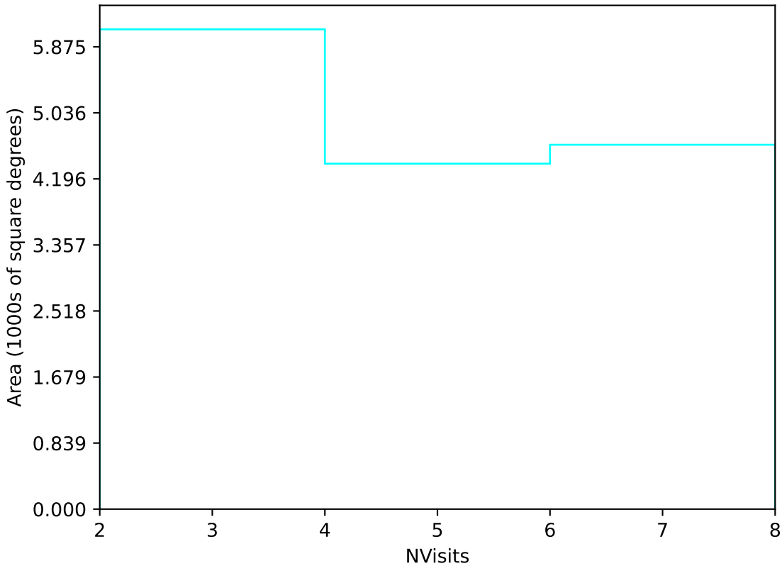
early_u_fpextra3.0_v3.4_10yrs Yr 3-4 u band: NVisits
