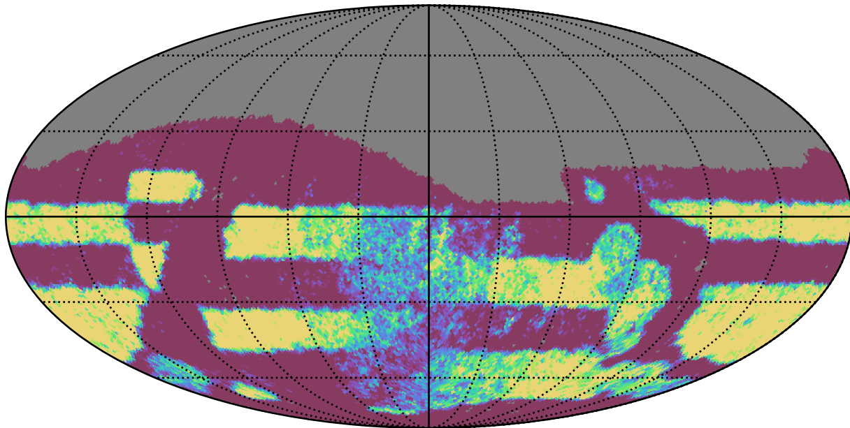
early_u_fpextra3.0_v3.4_10yrs Yr 3-4 r band: NVisits
