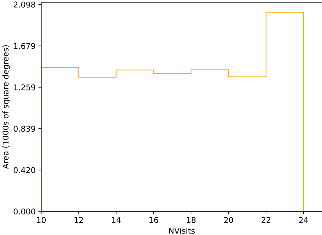
early_u_fpextra3.0_v3.4_10yrs Yr 3-4 r band: NVisits
