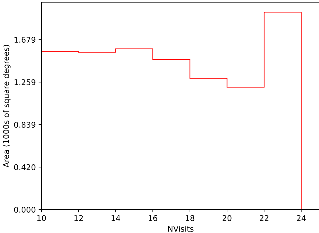
early_u_fpextra3.0_v3.4_10yrs Yr 3-4 i band: NVisits
