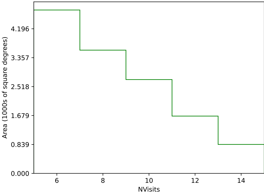
early_u_fpextra3.0_v3.4_10yrs Yr 3-4 g band: NVisits
