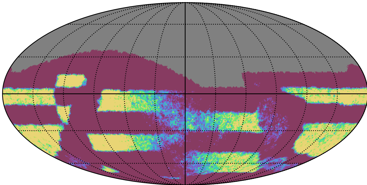
early_u_fpextra3.0_v3.4_10yrs Yr 3-4 all bands: NVisits
