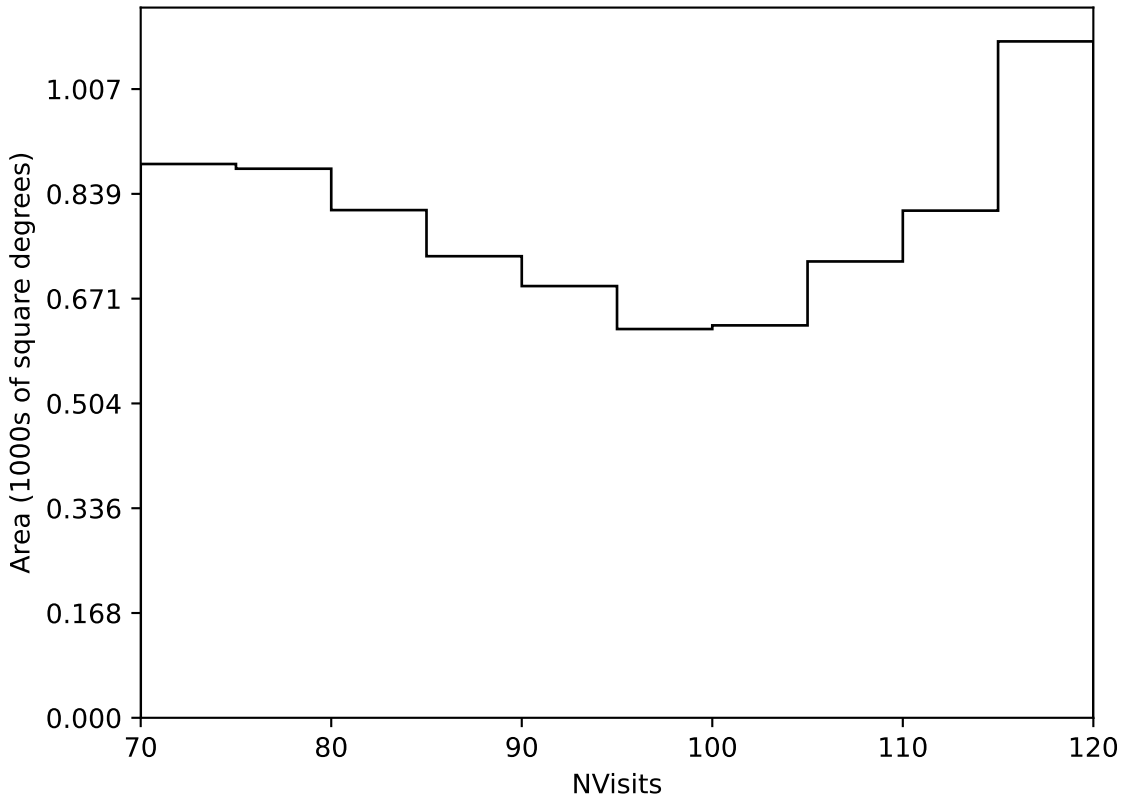
early_u_fpextra3.0_v3.4_10yrs Yr 3-4 all bands: NVisits
