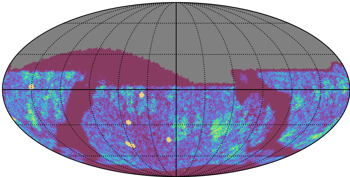
early_u_fpextra3.0_v3.4_10yrs Yr 1 z band: NVisits
