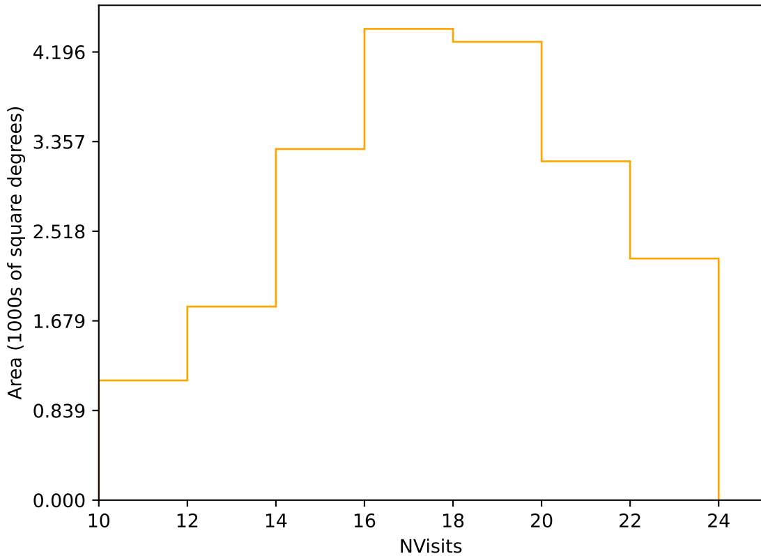
early_u_fpextra3.0_v3.4_10yrs Yr 1 r band: NVisits
