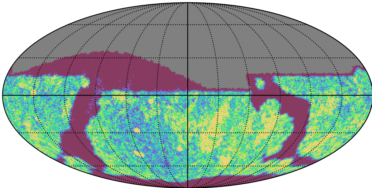
early_u_fpextra3.0_v3.4_10yrs Yr 1 i band: NVisits
