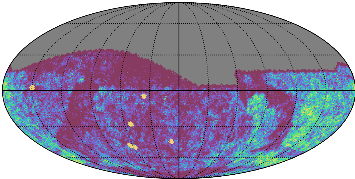
early_u_fpextra3.0_v3.4_10yrs Yr 1 g band: NVisits
