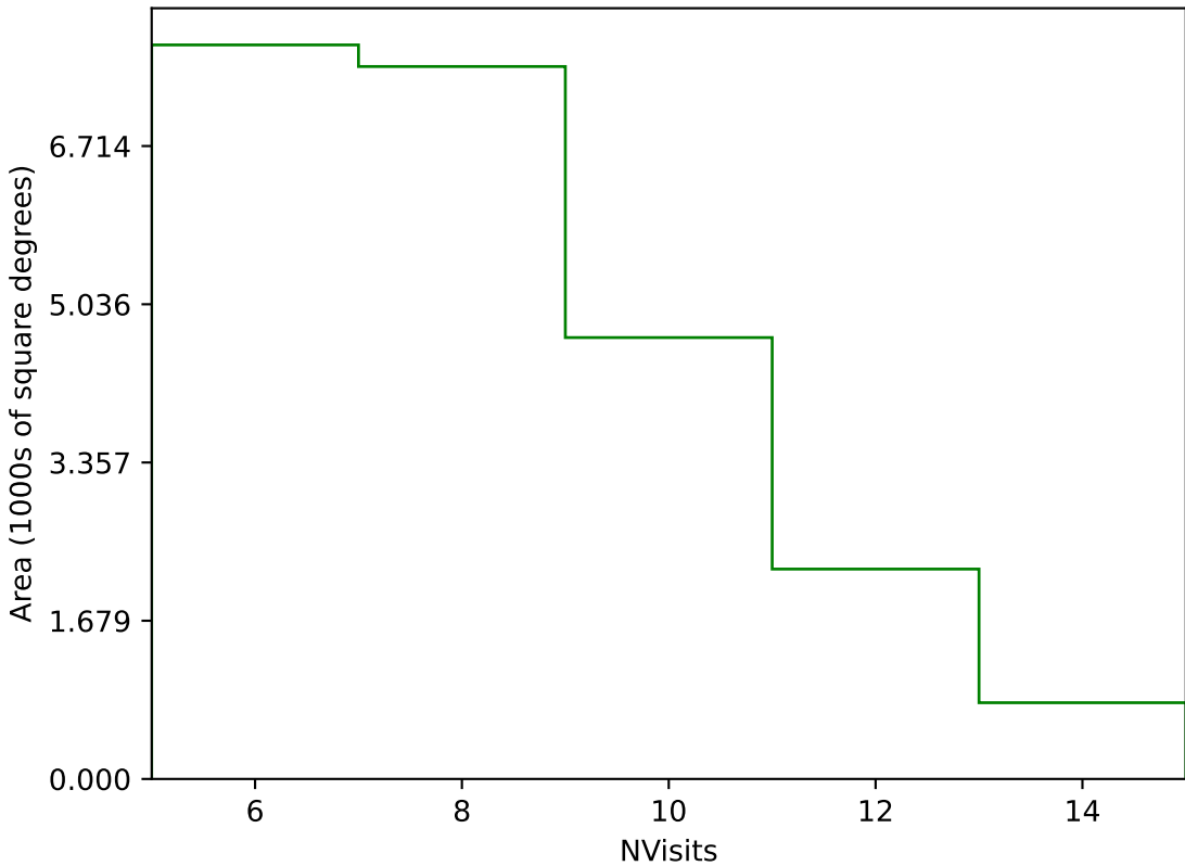
early_u_fpextra3.0_v3.4_10yrs Yr 1 g band: NVisits
